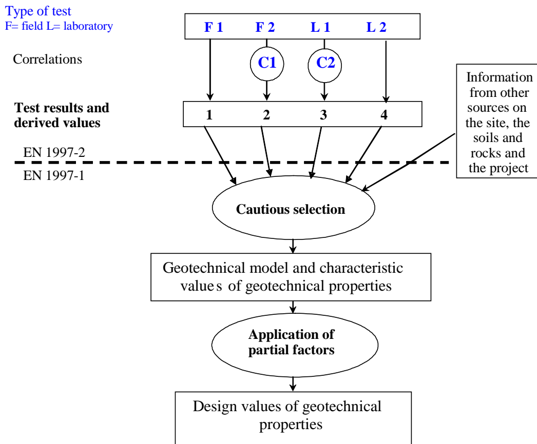
Figure. 1. General framework for the selection of derived values, characteristic values and design values of geotechnical properties (CEN, 2007)
