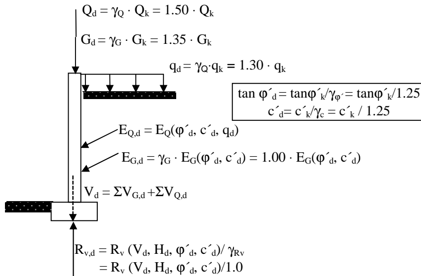
Figure 4. ULS in p&tds. Design Approach 3 - introduction of partial factors (recommended values) in the verification of ground bearing capacity (Frank et al., 2004).
