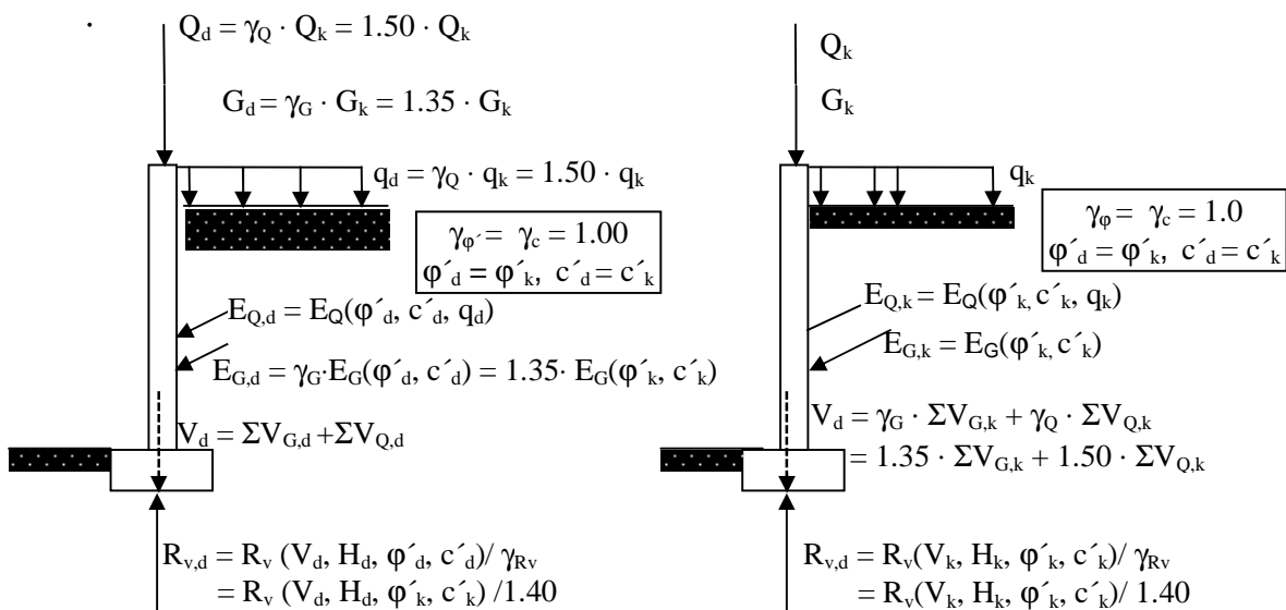
a) Factoring actions at the source (DA 2)
